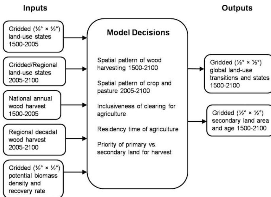
Figure 2. Flow diagram of inputs, outputs, and model decisions for the global land-use model (GLM) used in harmonisation. ▼
