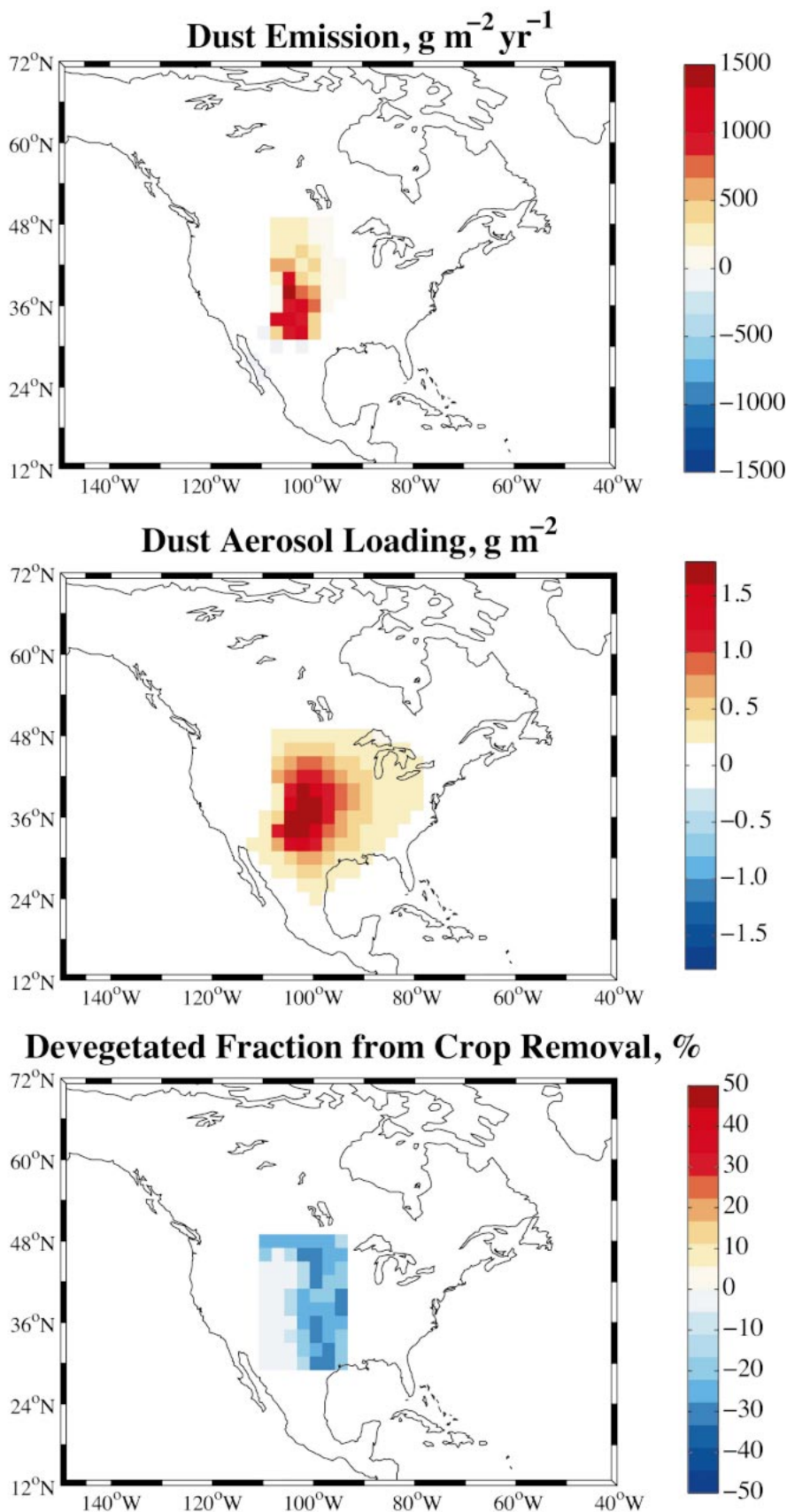
Figure 2. Dust emission (top, \text{g m}^{-2} \text{yr}^{-1} ) and dust aerosol loading (middle, \text{g m}^{-2} ) from the SST+DUST experiment and devegetated fraction (bottom, %) from the SST+CROP experiment, relative to SST-
