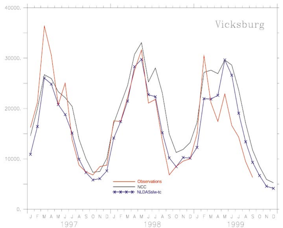
Figure 2. Time series of monthly mean streamflows ( \text{m}^3 \text{s}^{-1} ) at Vicksburg station, for the period 1997–
