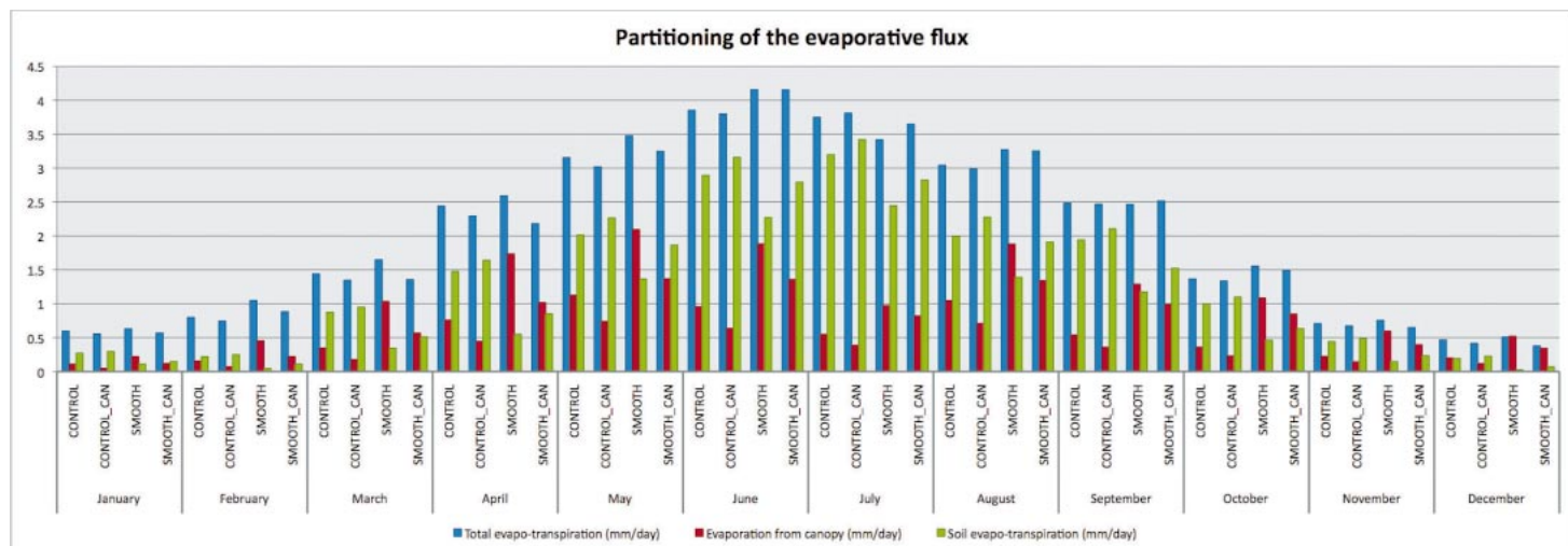
Figure 2. Annual cycle of total evapotranspiration (blue), in \text{mm day}^{-1} , partitioned into evaporation from canopy interception (red) and soil evaporation
