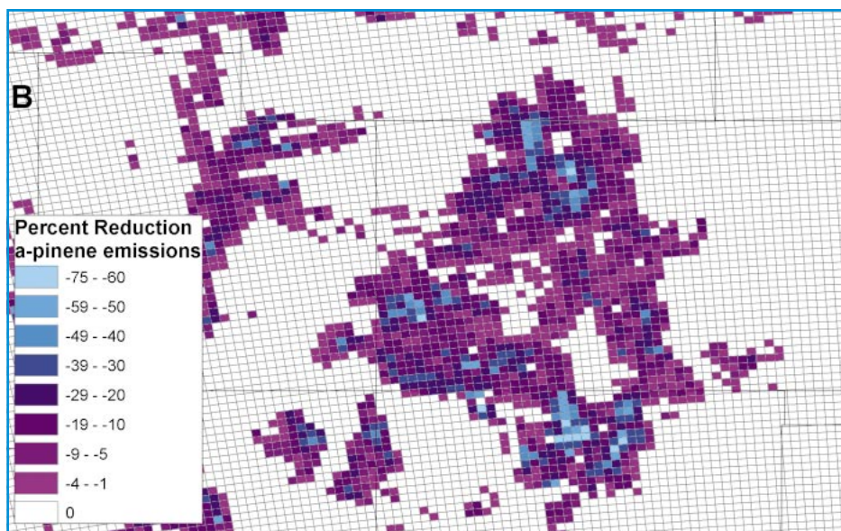
Figure 2B. The percent reduction in predicted biogenic \alpha -pinene emissions caused by a dieback of trees because of the insect infestation, assuming a short-term cessation of emissions.
