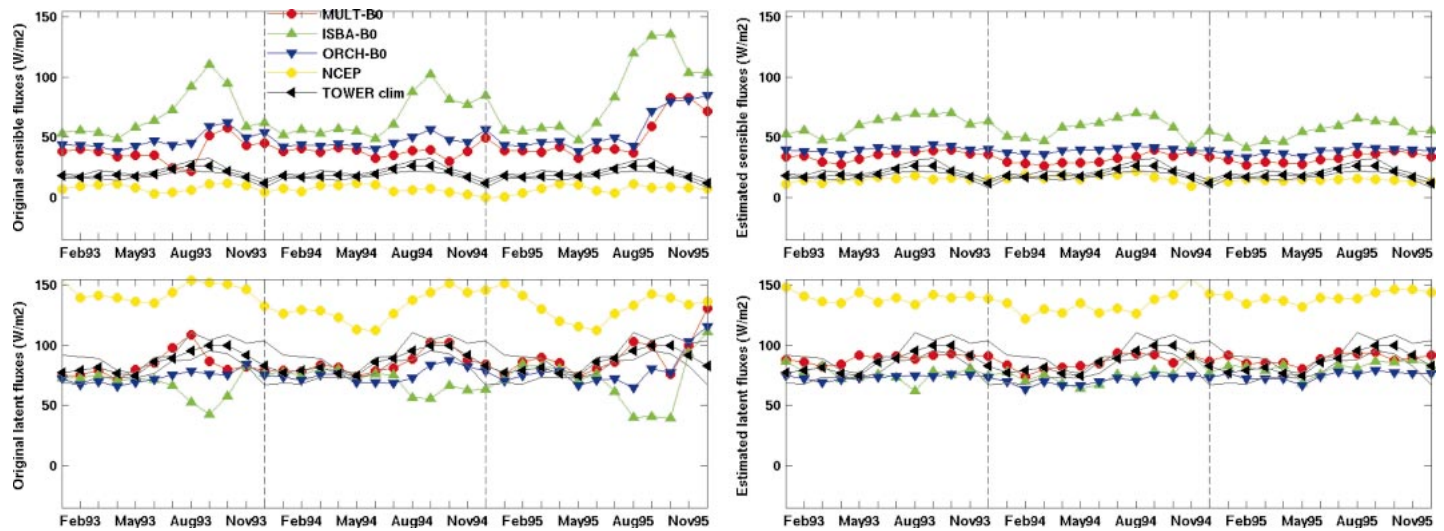
Figure 2. Averaged fluxes in a 2^{\circ} \times 2^{\circ} box around the Tapajos National Forest station near Santarém in Brazil ( 3^{\circ}\text{S} 55^{\circ}\text{W} ). Top left: the original LSM sensible heat flux; top right: the SM sensible heat flux; bottom left: the original LSM latent heat flux; and
