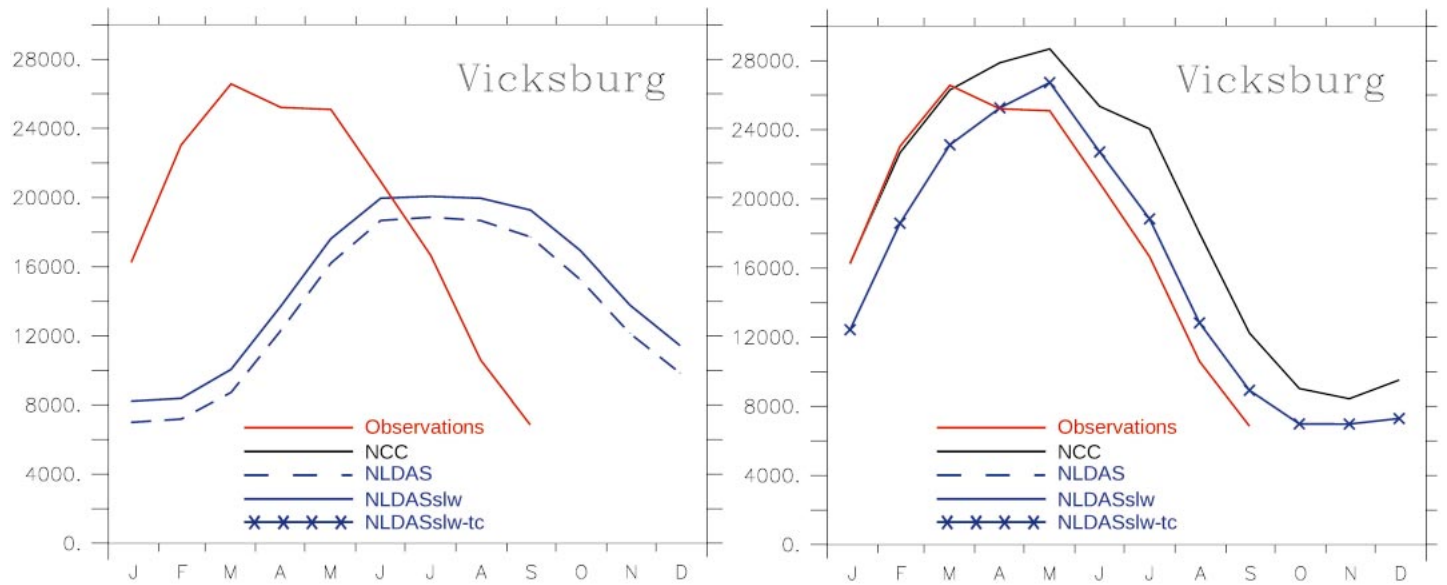
Figure 1. Monthly mean streamflows ( \text{m}^3 \text{s}^{-1} ) at Vicksburg station for the period 1997–1999 from
