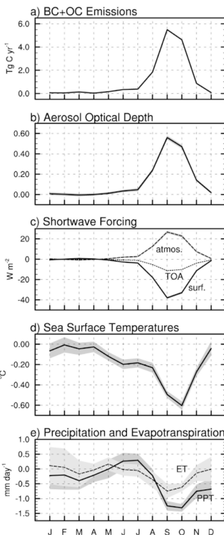
Figure 1. Observed climate forcing and simulated (CAM3) response to fire emissions in south-eastern Equatorial Asia (90°E-120°E, 5°S-5°N). a) observed fire emissions from the Global Fire Emissions Database (GFED), b) simulated aerosol optical depth, c) simulated net clear-sky shortwave radiation at the surface and through the troposphere (surface – 200 mbar) (W m -2 ), d) simulated sea surface temperatures (°C), and e) simulated evapotranspiration (ET, light line) and precipitation (PPT, dark line) (mm d -1 ).
